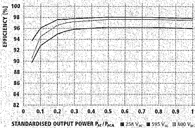
FRONIUS SYMO 8.2-3-M EFFICIENCY CURVE
