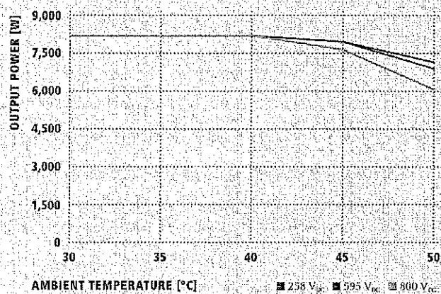
FRONIUS SYMO 8.2-3-M TEMPERATURE DERATING
